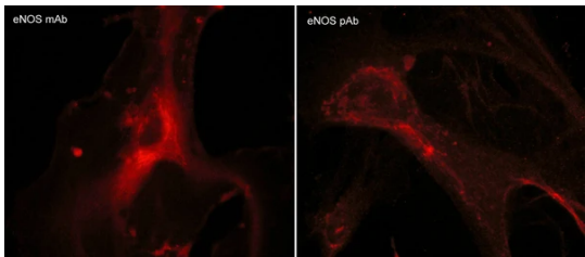
Immunocytochemical labeling of endothelial nitric oxide synthase (eNOS) in paraformaldehyde-fixed and NP-40-permeabilized human umbilical vein endothelial cells. The cells were labeled with mouse monoclonal eNOS (NM2211) and rabbit polyclonal eNOS (NP2281) antibodies, then the antibodies were detected using appropriate secondary antibodies conjugated to Cy3.
