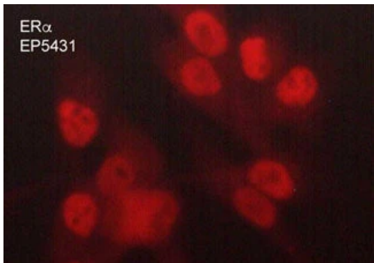
Immunocytochemical labeling of Estrogen Receptor α in paraformaldehyde fixed and NP-40 permeabilized MDA-MB-231 cells. The cells were labeled with rabbit polyclonal anti-Estrogen Receptor α (EP5431). The antibody was detected using goat anti-rabbit DyLight® 594.
