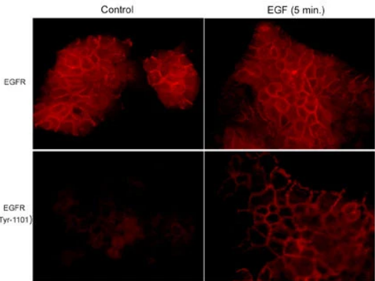
Immunocytochemical labeling in A431 cells untreated or treated with EGF (100 ng/ml) for 5 min. The cells were labeled with mouse monoclonals anti-EGFR (EM1661) and anti-EGFR (Tyr-1101) (EM1991).
