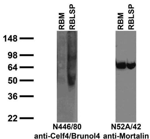
Adult rat brain membrane (RBM) and low-speed pellet (RBLSP) immunoblot.
